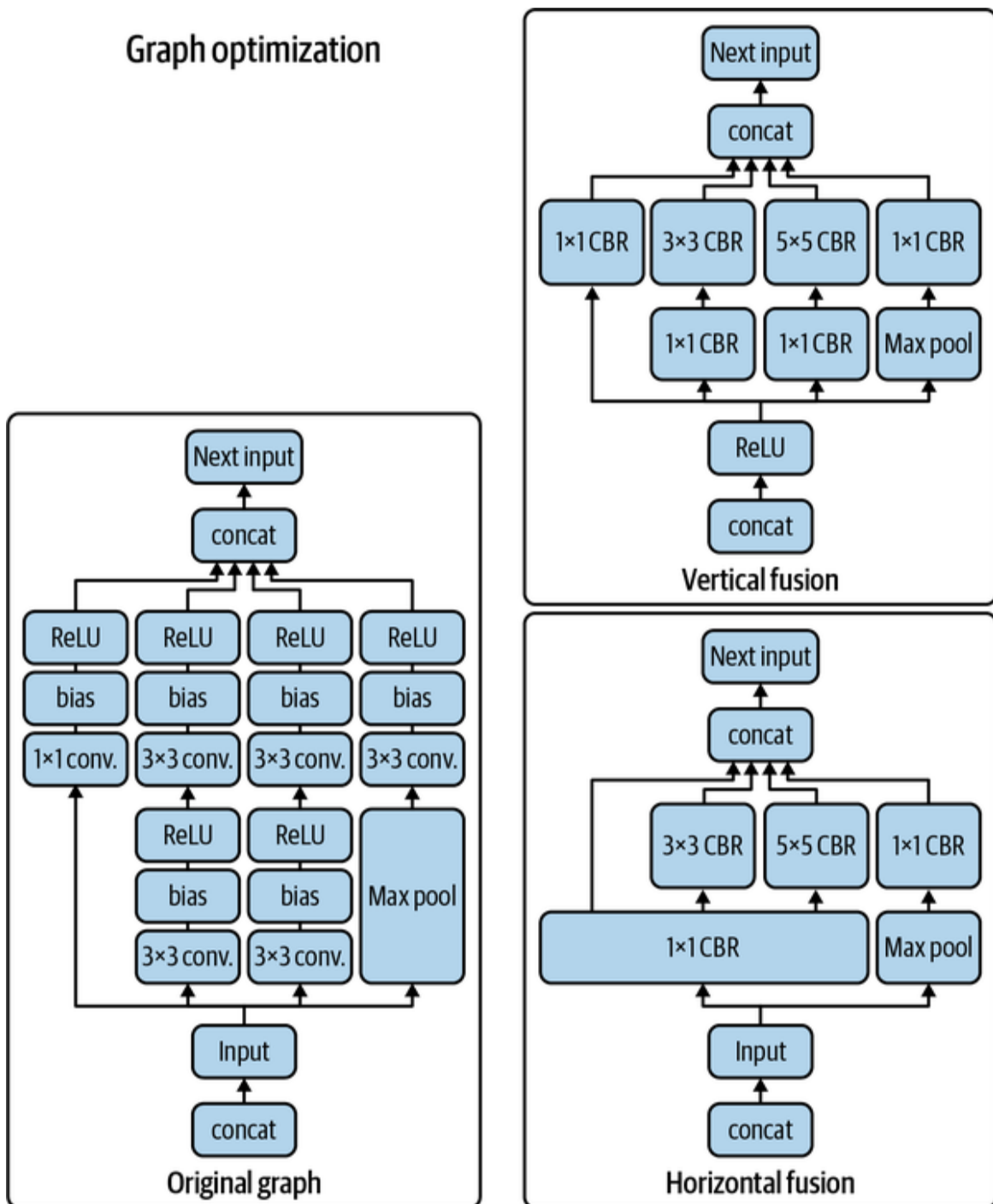
Figure 7-14. Vertical and horizontal fusion of the computation graph of a convolution neural network. Source: Adapted from an image by TensorRT team 48
